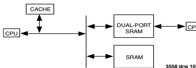
Flow Chart 4. Dual-Port SRAM in a Cached Memory Environment
